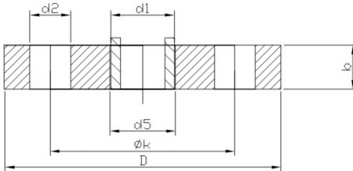
Slip-on Flange 6 bar
